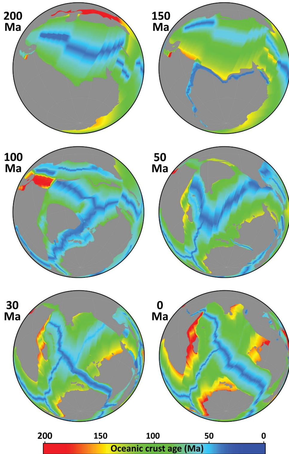
Figure 2: Oblique view of the oceanic crustal age of the Indian Ocean region since 200 Ma to present day, showing the break-up of Eastern Gondwana continent and opening of the Indian Ocean. Images created using gPlates software ( https://www.earthbyte.org/category/resources/software-workflows/pygplates/ ). Base maps are from Müller et al. 2019.
