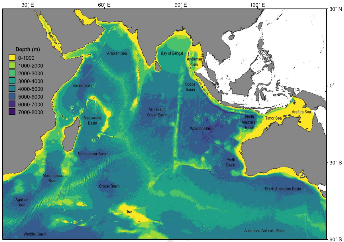
Figure 3: Bathymetric map of the Indian Ocean with major basins and seas labelled. Note that the Persian Gulf to the north is not included in this study as it is shallower than 1,000 m.
