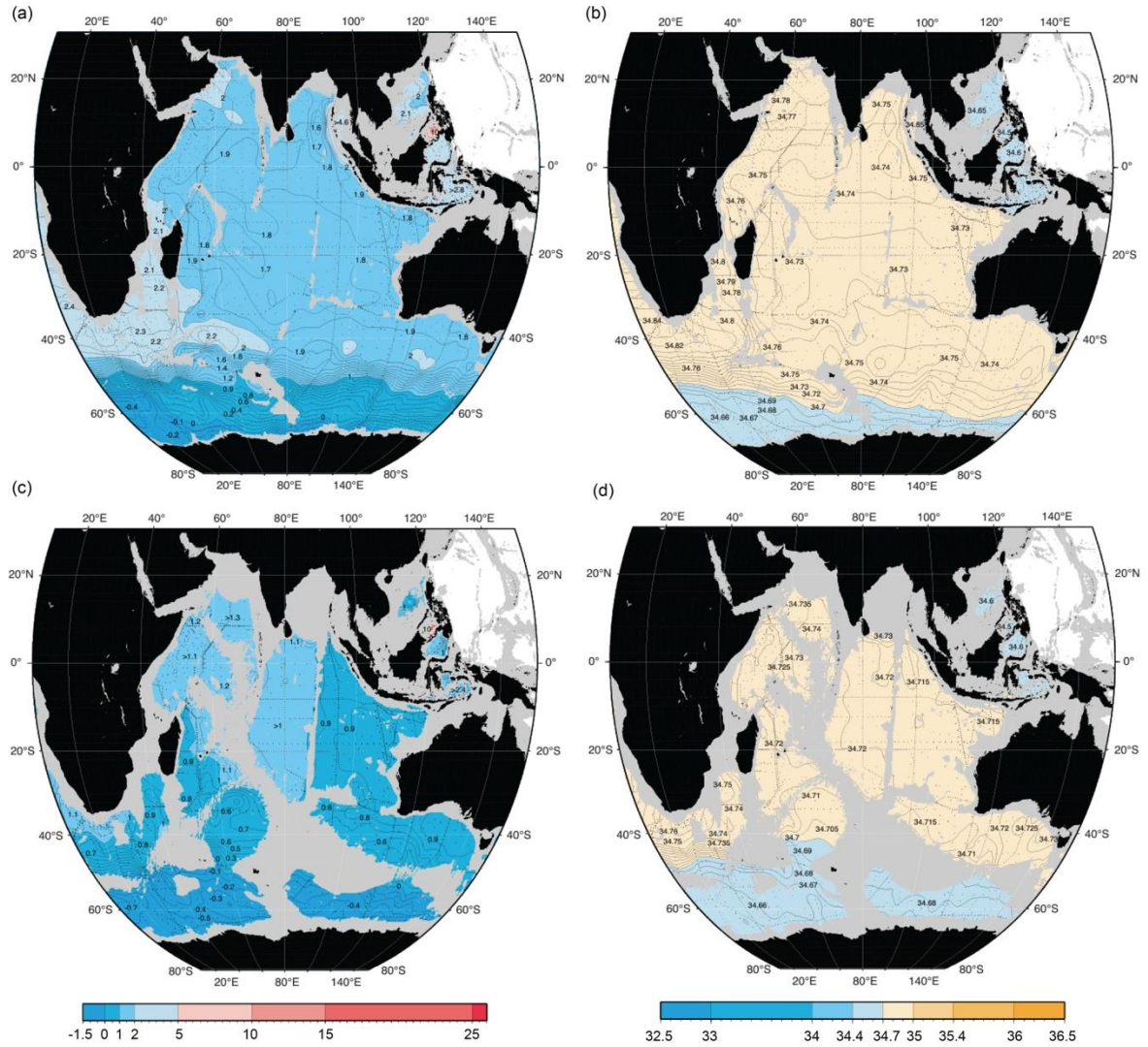
Figure 4: Deep and bottom water properties of the Indian Ocean from the World Ocean Circulation Experiment Indian Ocean Atlas (Talley 2013). (a) Potential Temperature (°C) and (b) Practical Salinity at 2,500 m, (c) Potential Temperature (°C) and (d) Practical Salinity at 4,000 m.
