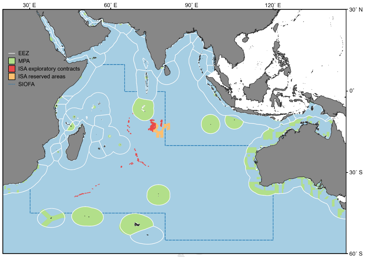
Figure 1: Map of the Indian Ocean with exclusive economic zone (EEZ) boundaries of neighbouring countries (white lines), SIOFA management area (blue dashed lines), established marine protected areas (MPAs, green polygons), and International Seabed Authority (ISA) exploratory mining contracts (red polygons) and reserved areas (orange polygons). The blue area defines the limits of the Indian Ocean.
