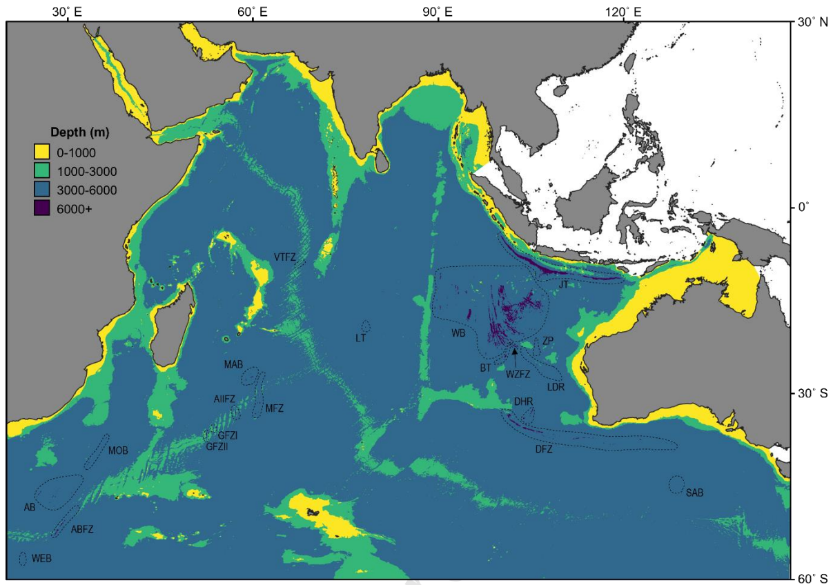
Figure 10: Hadal features of the Indian Ocean, with hadal depths > 6,000 m and hadal features marked by dashed lines. AB: Agulhas Basin, ABFZ: Andrew Bain Fracture Zone, AIFZ: Atlantis II Fracture Zone, BT: Brouwer Trough, DFZ: Diamantina Fracture Zone, DHR: Dirck Hartog Ridge, GFZI: Gazelle Fracture Zone, GFZII: Gallieni Fracture Zone, JT: Java Trench, LDR: Lost Dutchmen Ridge, LT: Langseth Trough, MAB: Madagascar Basin, MFZ: Melville Fracture Zone, MOB: Mozambique Basin, SAB: South Australian Basin, VTFZ: Vema Trench Fracture Zone, WB: Wharton Basin, WEB: Weddell Basin, WZFZ: Wallaby-Zenith Fracture Zone, ZP: Zenith Plateau.
